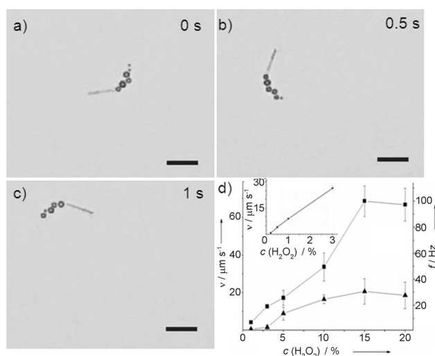
Figure 2. a)–c) Time-lapse images of the motion of a (CHI/ALG) 18 -PtNP nanorocket in 15 % \text{H}_2\text{O}_2 solution recorded by using an optical microscope at 22 °C. Scale bars: 10 \mu\text{m} . d) The dependence of the average speed v of (CHI/ALG) 18 -PtNP nanorockets (▲) and the frequency f of bubbles (■) on \text{H}_2\text{O}_2 concentration c(\text{H}_2\text{O}_2) in the range of 1–20 % at 22 °C. Inset: The dependence of the nanorocket speed on low \text{H}_2\text{O}_2 concentration at 37 °C.
